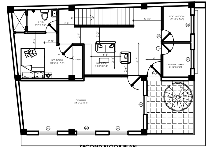
SECOND FLOOR PLAN AREA:931.90 SQ. FT
