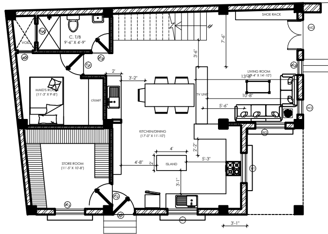
GROUND FLOOR PLAN AREA:1045.95 SQ.FT
